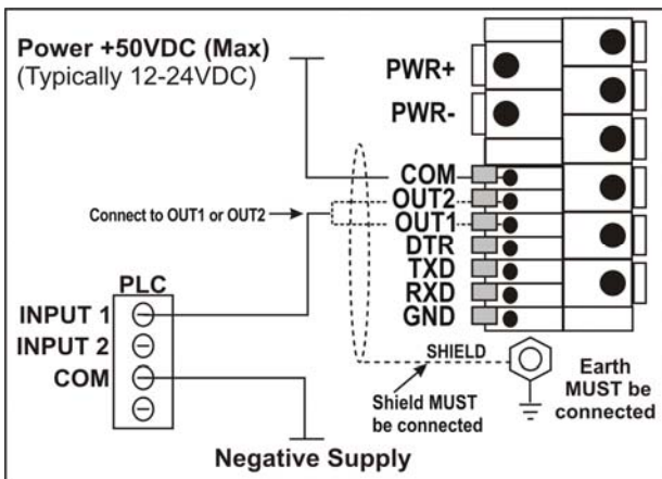
Figure 10: Instrument Outputs to Drive PLC
